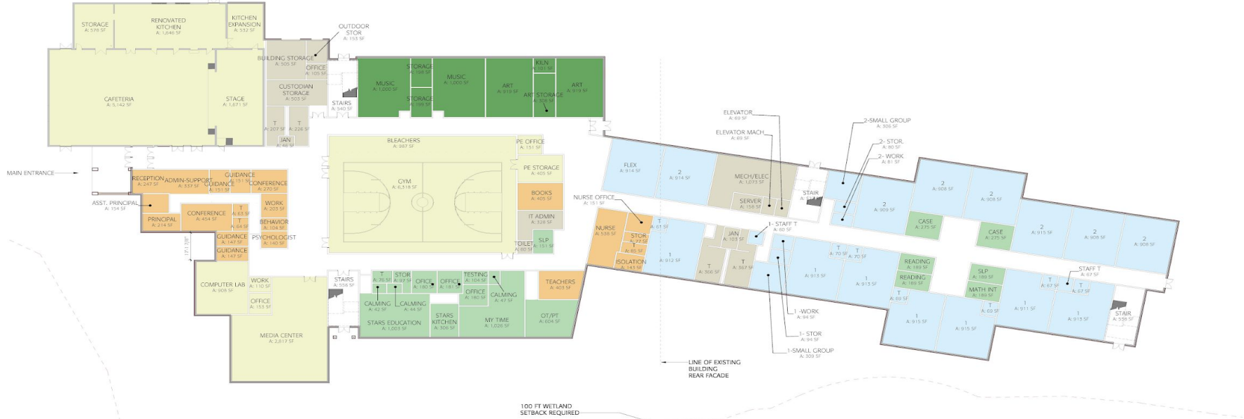
OPTION 2 FIRST FLOOR PLAN 1"=20'
